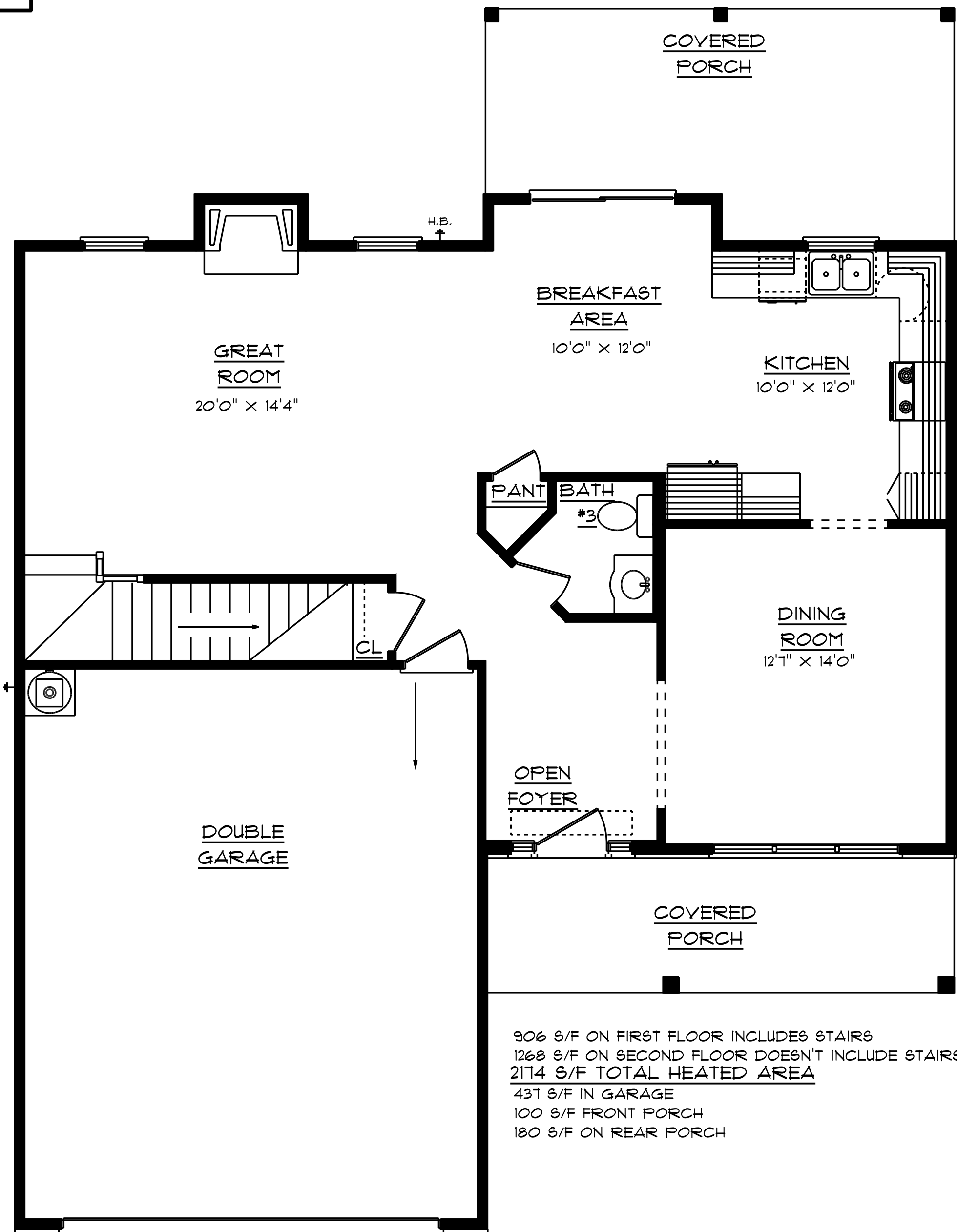
FIRST FLOOR
