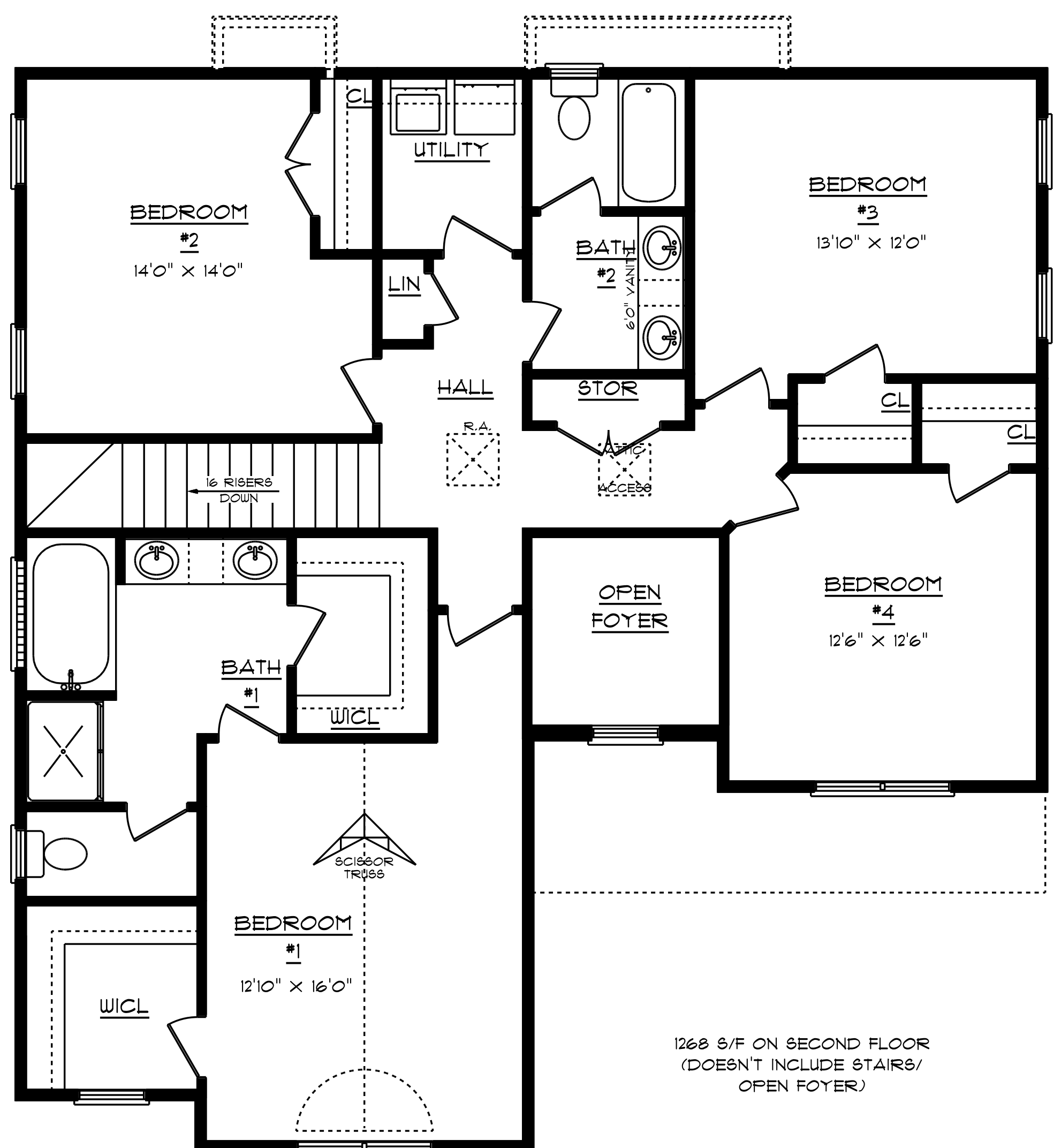
SECOND FLOOR
